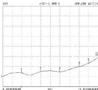
S11 FORWARD REFLECTION
